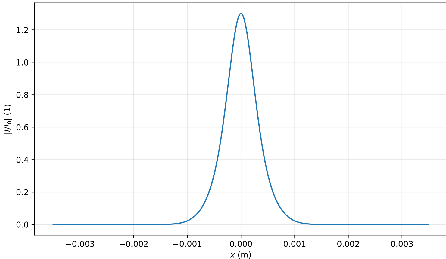
Intensity profile I(x, y = 0, z = 0.796m)/I_0 , P_{in}=0.9P_{cr} , artificial time
